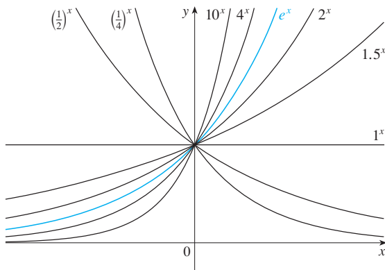
Exponential functions
