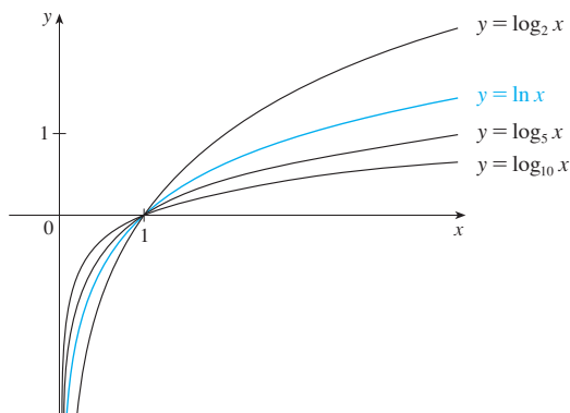
Logarithmic functions
